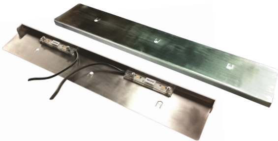
Model IL618.150.500 18.0" width x .5" height x 3.0" depth Includes two 2.0 watt LED modules
